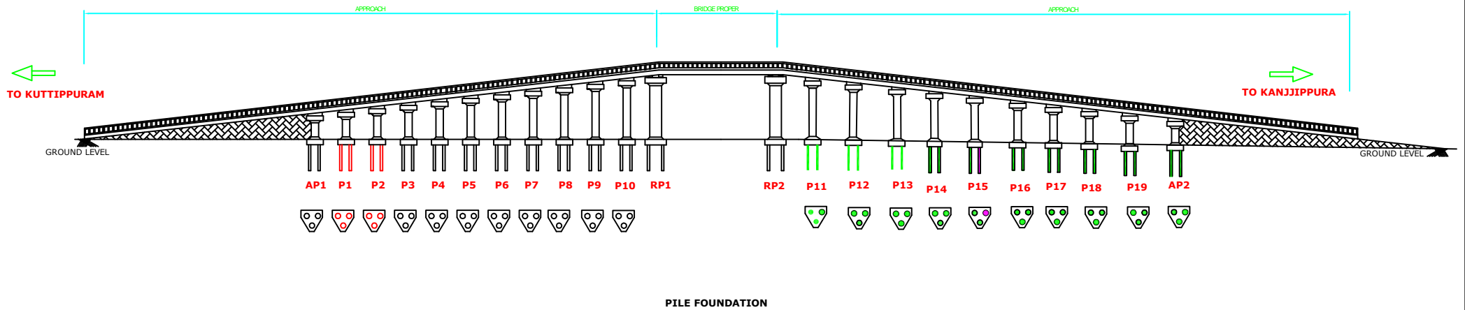
PILE FOUNDATION
